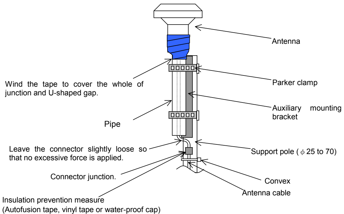
Figure 6.3.1 An Example of Installation, Using GPA-017S for Antenna
